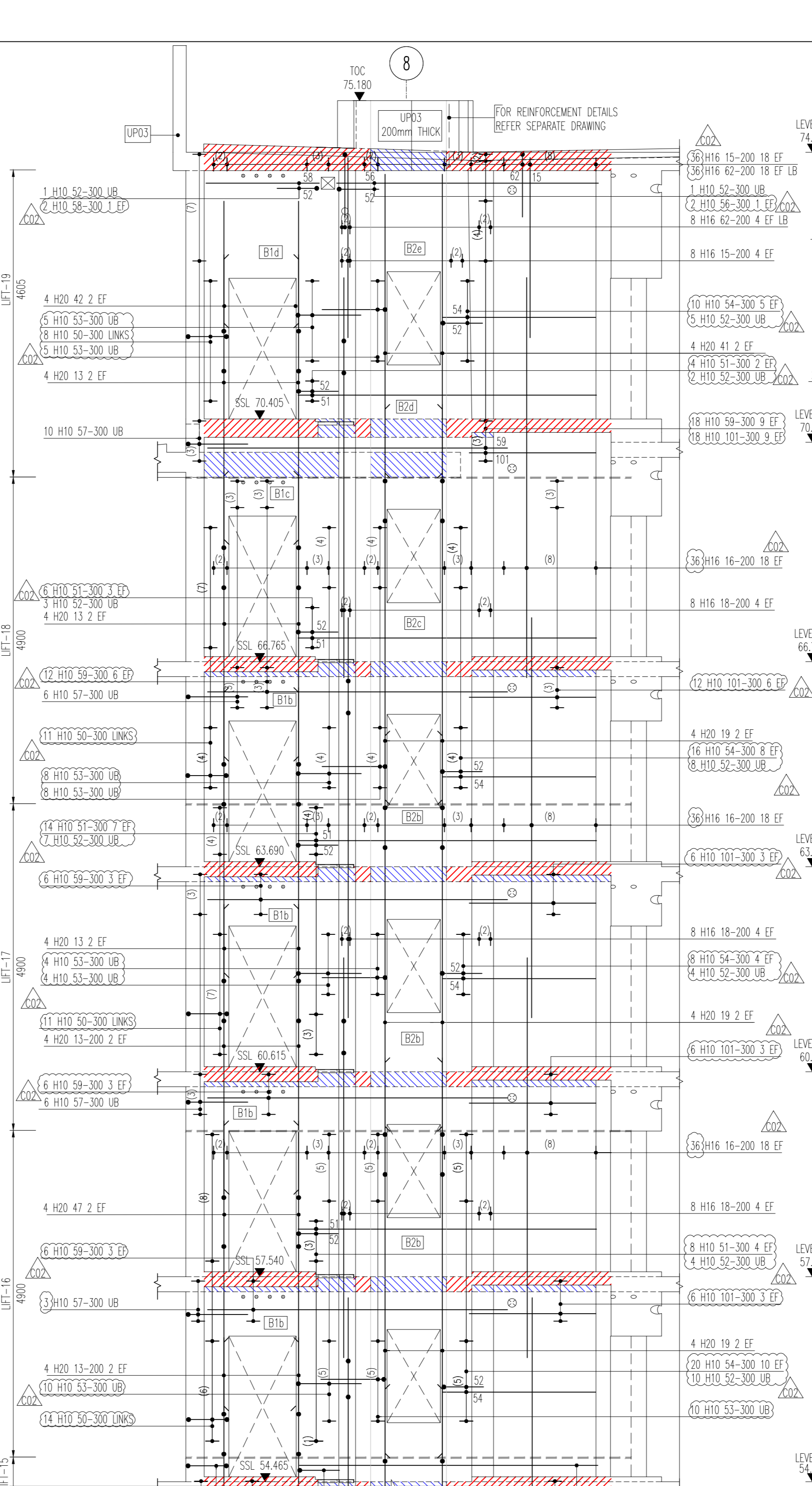
WALL 19 LEVEL 15 TO ROOF (300mm THICK WALL) SCALE 1:50
